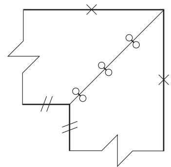
Full Mitre Joint
